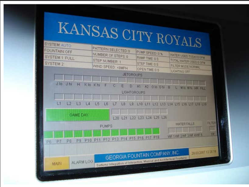
GEFCO Select #EE140 Animation Computer Interface with fiber-optic communications
