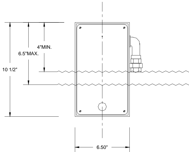
SCALE: NONE DIMENSIONS SUBJECT TO CHANGE WITHOUT NOTICE
