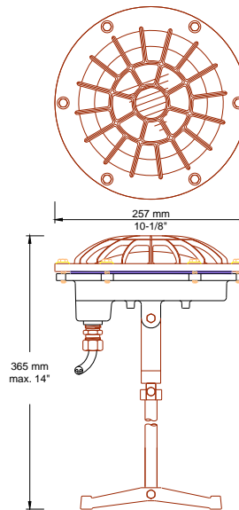
Shown with optional rock guard and stand
