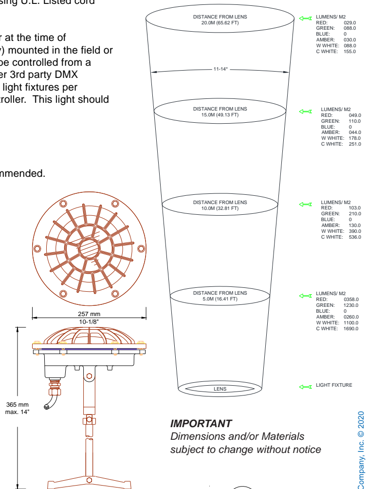
Shown with optional rock guard and stand
